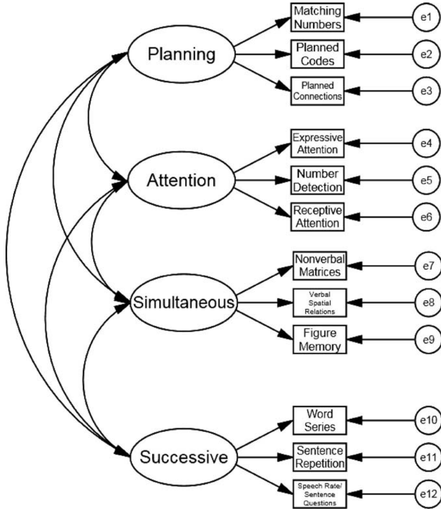
Figure 1. Cognitive Assessment System factor structure tested through multigroup confirmatory factor analysis.
